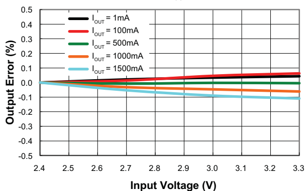
Line Regulation ( L = 2.2\mu\text{H} , V_{\text{OUT}} = 3.8\text{V} )
