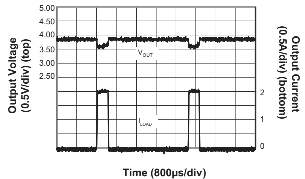
Figure 2: AAT2215 Operation Waveform When 2.0A 217Hz 577 \mu s Load Pulse is Applied.
